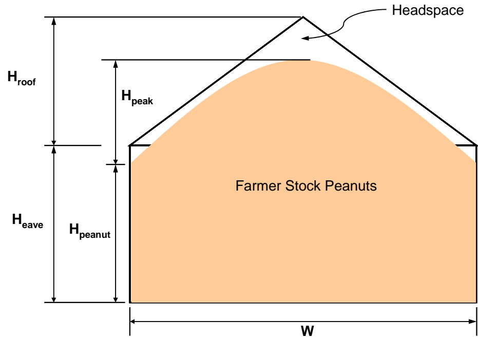
Figure 2. Warehouse cross-section for ventilation calculation example.
