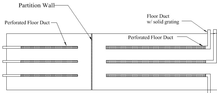
Figure 3. Typical farmer stock peanut warehouse with aeration floor plan.
