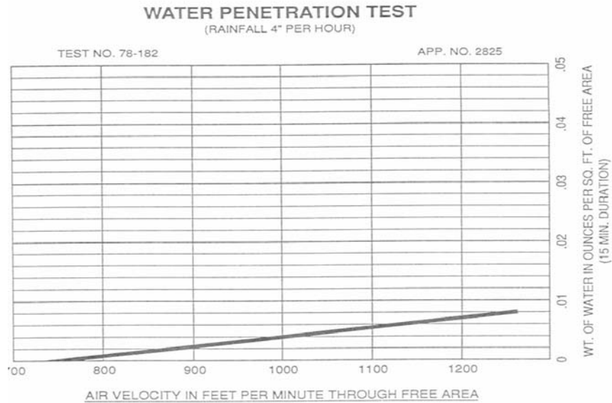
Figure 1. Amount of water carried into a test structure at various inlet air velocities.
